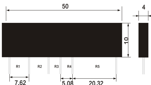
TC1766A LAYOUT UNIT: mm R1=1K R2=9K R3=90K R4=900K R5=9M
