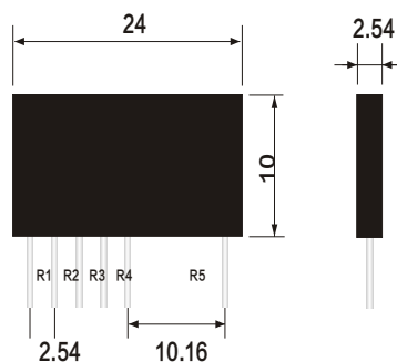
TC1746A LAYOUT UNIT: mm R1=1K001 R2=10K01 R3=100K01 R4=1M1111 R5=10M
