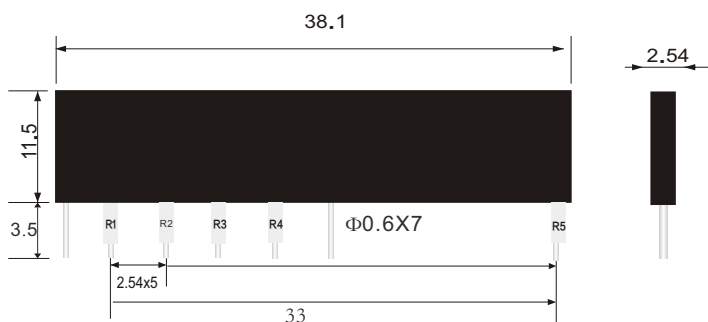
TC1786A LAYOUT UNIT: mm R1=1.0001K R2=10.01K R3=101.01K R4=1.1111M R5=10.0000M
